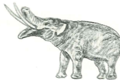
GNATHABELODON
