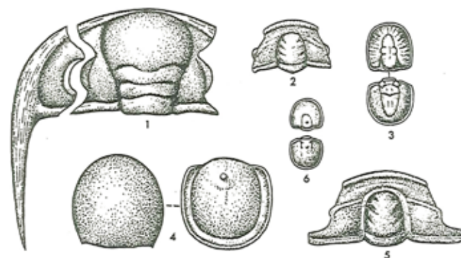
Figur 8. Mellem-kambriske trilobiter fra Bornholm. 1: Paradoxides (Exsulans-kalk), 2: Jincella (Exsulans-kalk), 3: Ptychagnostus (Nedre alunskifer), 4: Grandagnostus (Andrarum-kalk), 5: Jincella (Andrarum-kalk), 6: Lejopyge (Øvre alunskifer).
