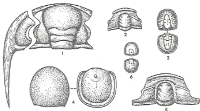
Figur 22. Mellem Kambriske trilobitter fra Bornholm. 1: Paradoxides ('Exsulans Kalk'), 2: Jincella ('Exsulans Kalk'), 3: Ptychagnostus (nedre alunskifer), 4: Grandagnostus (Andrarum Kalk), 5: Jincella (Andrarum Kalk), 6: Lejopyge (øvre alunskifer).
