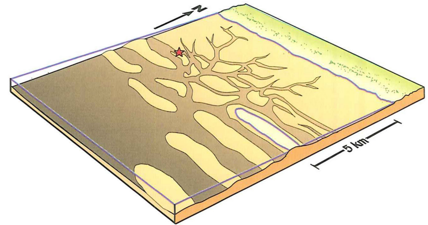
Figur 6a. Aflejringsmiljø for Vik member
